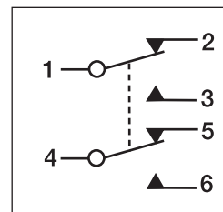
2PDT Schematic
