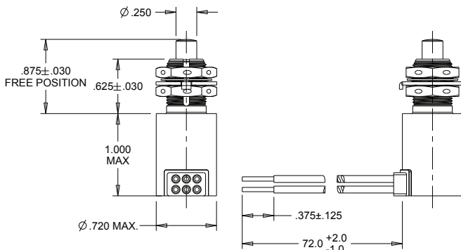
Style A Pin Plunger Radial Leads
