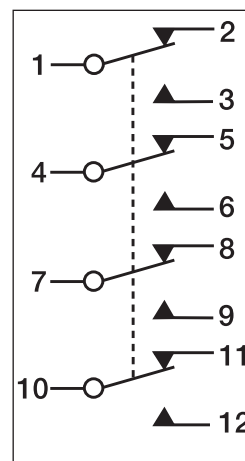
4PDT Schematic
