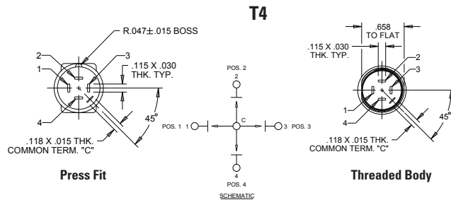
Threaded Body
