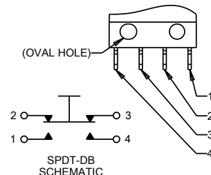
CIRCUIT STYLE 4 SPDT-DB, FORM Z
