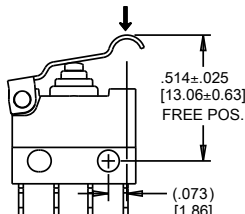
"U" SHAPED LEVER (LEVER TYPE OPTION 2)
