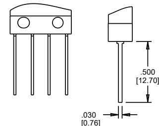
TERMINAL STYLE 4 WIRE WRAP
