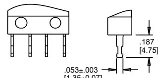
TERMINAL STYLE 3 TURRET, 3/16" LONG
