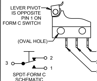
CIRCUIT STYLE 3 SPDT, FORM C
