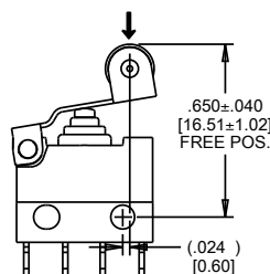
IN-LINE ROLLER LEVER (LEVER TYPE OPTION 3)
