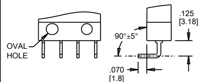
TERMINAL STYLE 5 RIGHT ANGLE PC PINS
