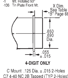
Figure 8. C & C7 MOUNTS
