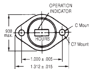
Figure 8. C & C7 MOUNTS
